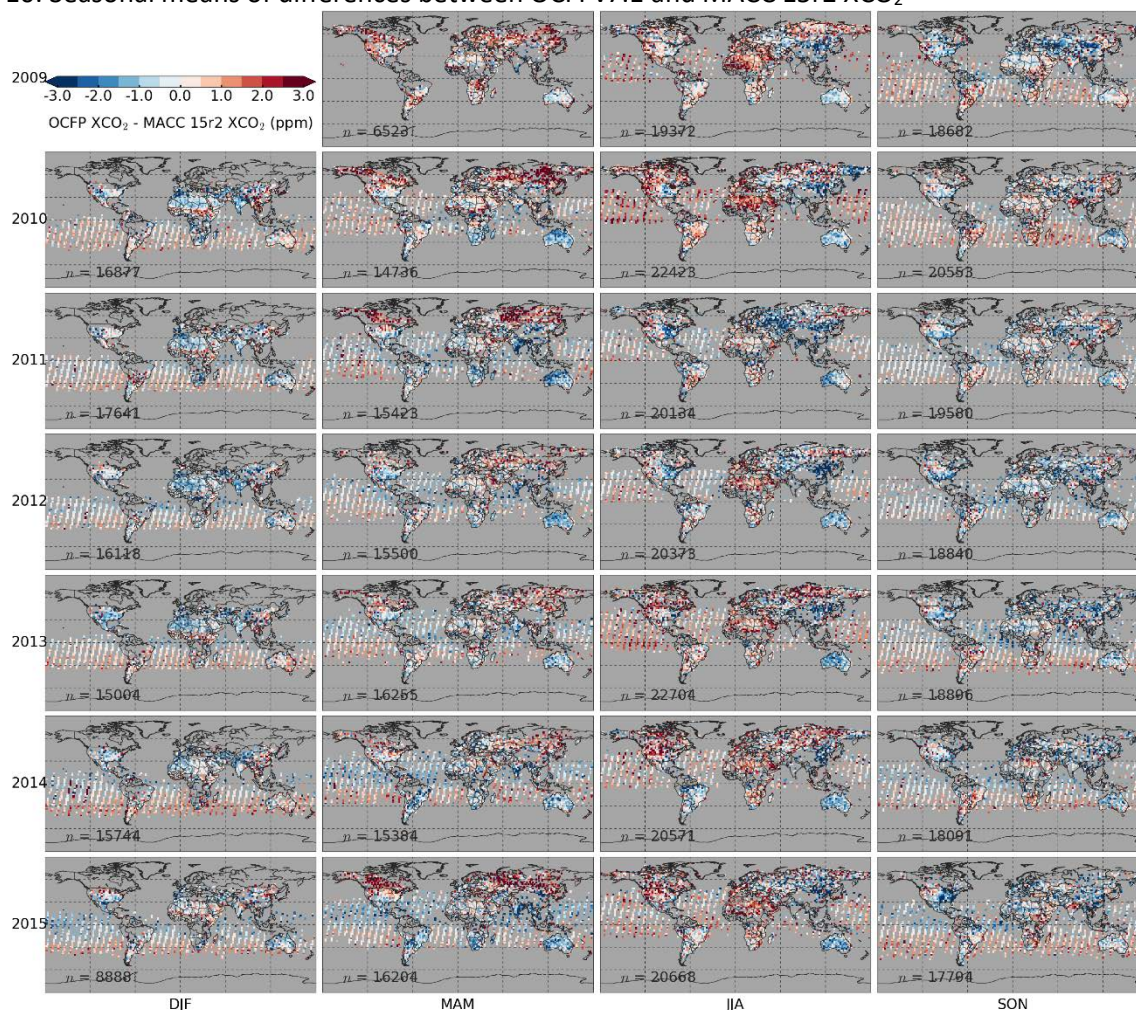
Figure 10: Seasonal means of differences between OCFPv7.1 and MACC 15r2 XCO 2
