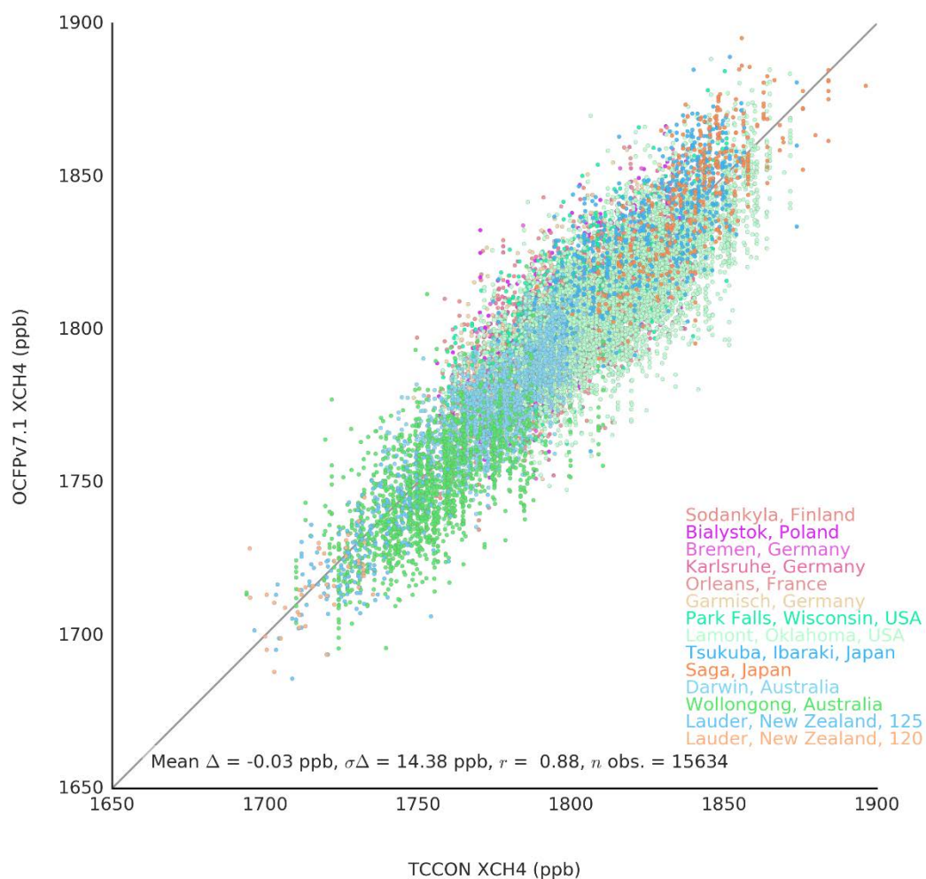
Figure 4: Correlation of TCCON GGG2014 and OCFPv7.1 XCH 4 observations over all TCCON sites mentioned in Table 2.
