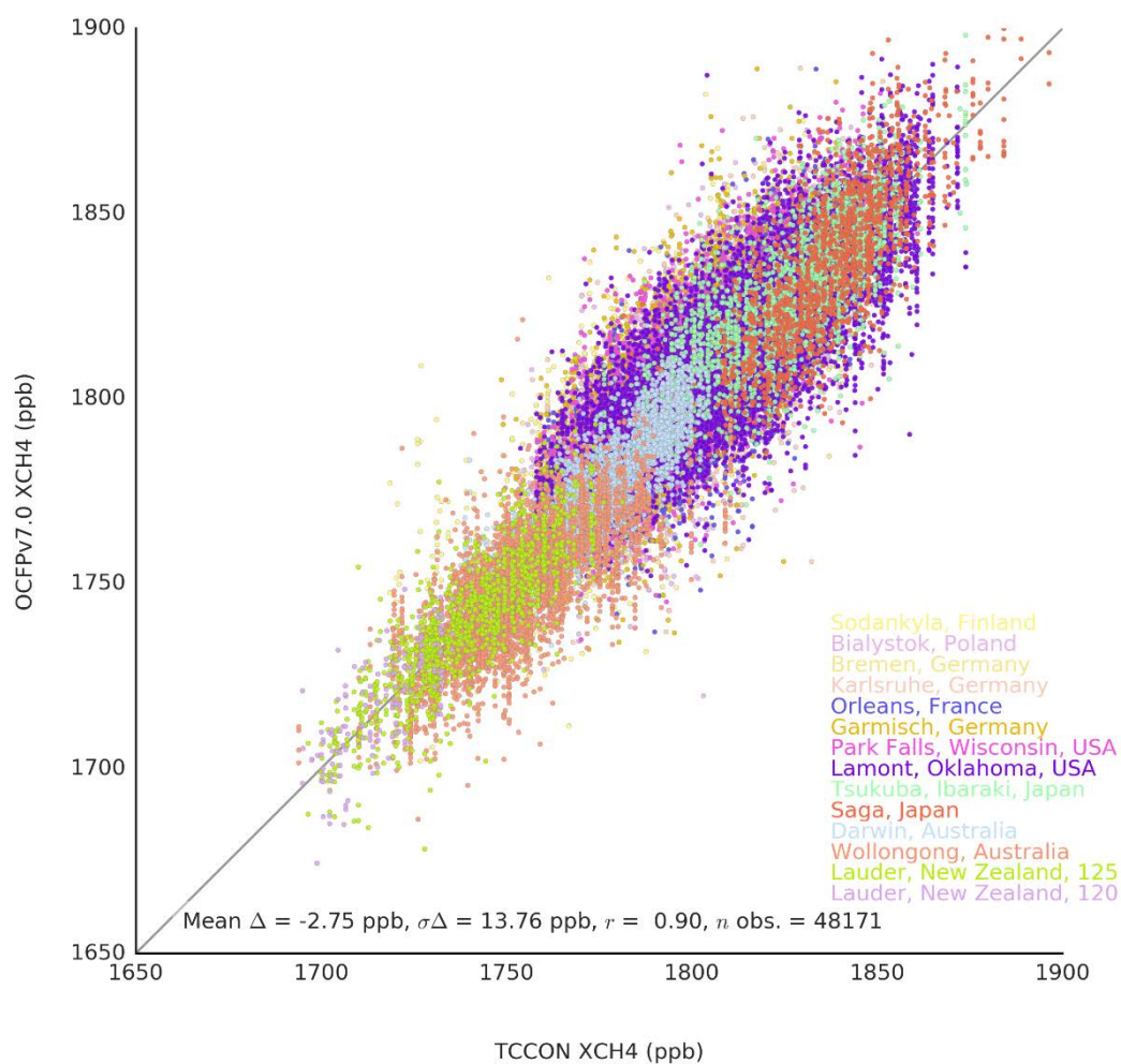
Figure 7: Correlation of TCCON GGG2014 and OCFPv7.0 XCH 4 observations over all TCCON sites mentioned in Table 2.
