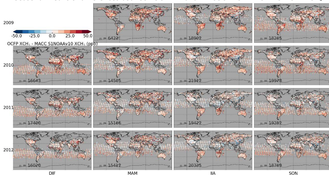
Figure 11: Seasonal means of differences between OCFP7.1 and MACC S1NOAAv10 + TOMCAT XCH 4
