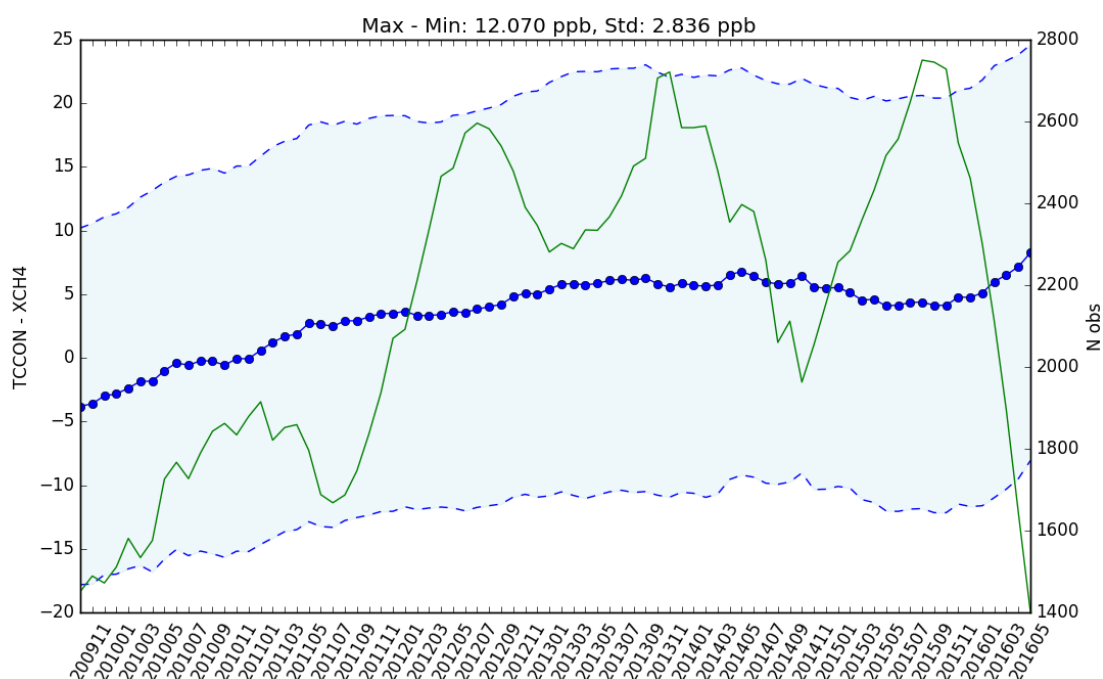
Figure 6: Year-to-year Stability of the TCCON-OCFPv7.1 XCH 4 bias calculated with for \pm 6 month averaging window for each month of the GOSAT time series between April 2009 and December 2016. The thick blue symbols give the mean bias for a 12 month period and the shaded area indicates the standard deviation (1-sigma) of the data. The green lines gives the number of data points per 12 month period.
