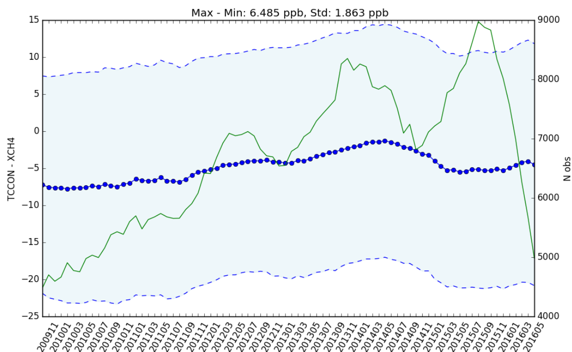
Figure 9: Year-to-year Stability of the TCCON-OCPv7.1 XCH 4 bias calculated with for \pm 6 month averaging window for each month of the GOSAT time series between April 2009 and December 2016. The thick blue symbols give the mean bias for a 12 month period and the shaded area indicates the standard deviation (1-sigma) of the data. The green lines gives the number of data points per 12 month period.
