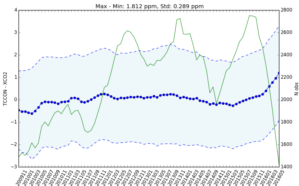
Figure 3: Year-to-year Stability of the TCCON-OCFPv7.1 XCO 2 bias calculated with for \pm 6 month averaging window for each month of the GOSAT time series between April 2009 and December 2016. The thick blue symbols give the mean bias for a 12 month period and the shaded area indicates the standard deviation (1-sigma) of the data. The green lines gives the number of data points per 12 month period.
