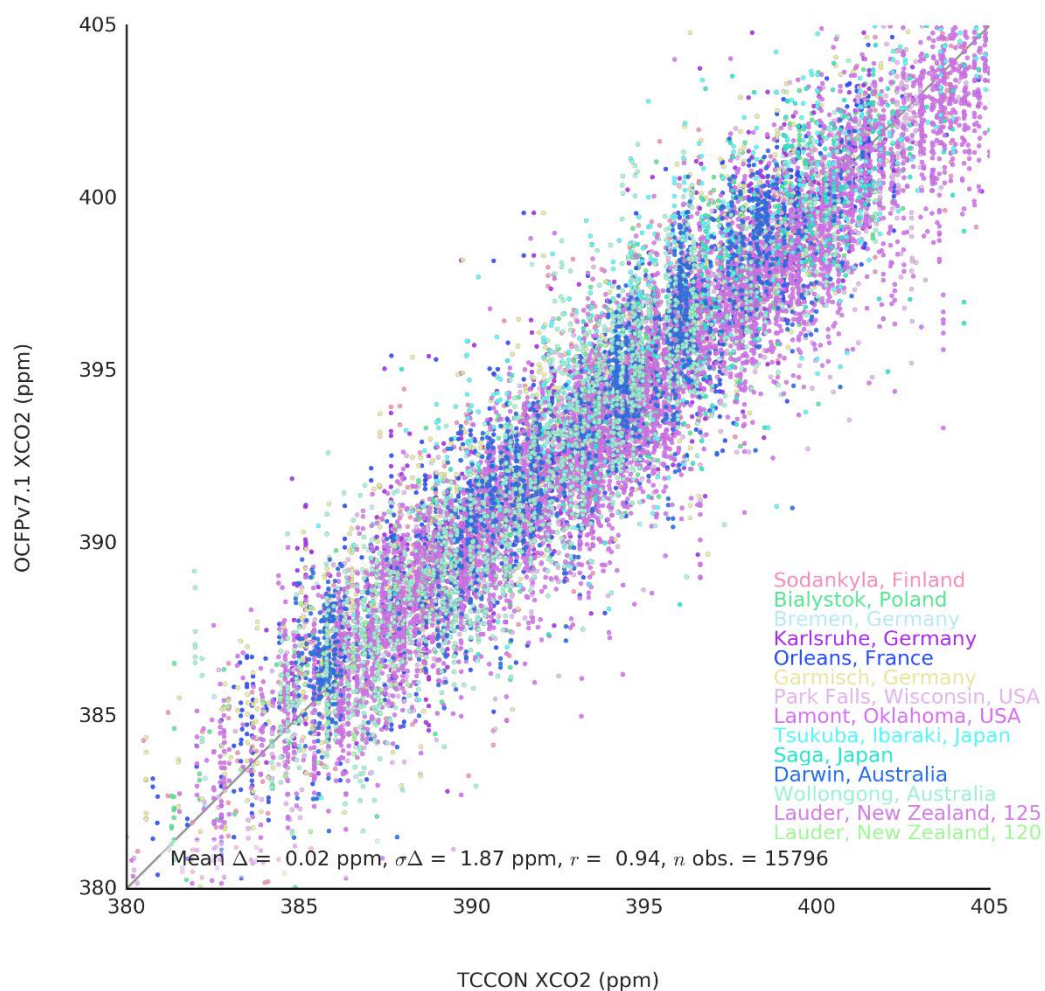
Figure 1: Correlation of TCCON GGG2014 and OCFPv7.1 XCO 2 observations over all TCCON sites mentioned in Table 2.
