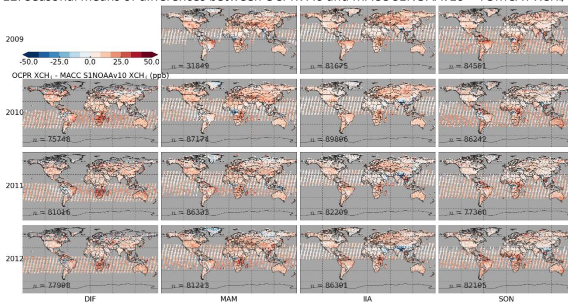
Figure 12: Seasonal means of differences between OCPv7.0 and MACC S1NOAAv10 + TOMCAT XCH 4
