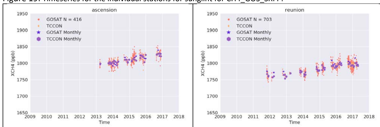
Figure 19: Timeseries for the individual stations for sunglint for CH4_GOS_SRF.
