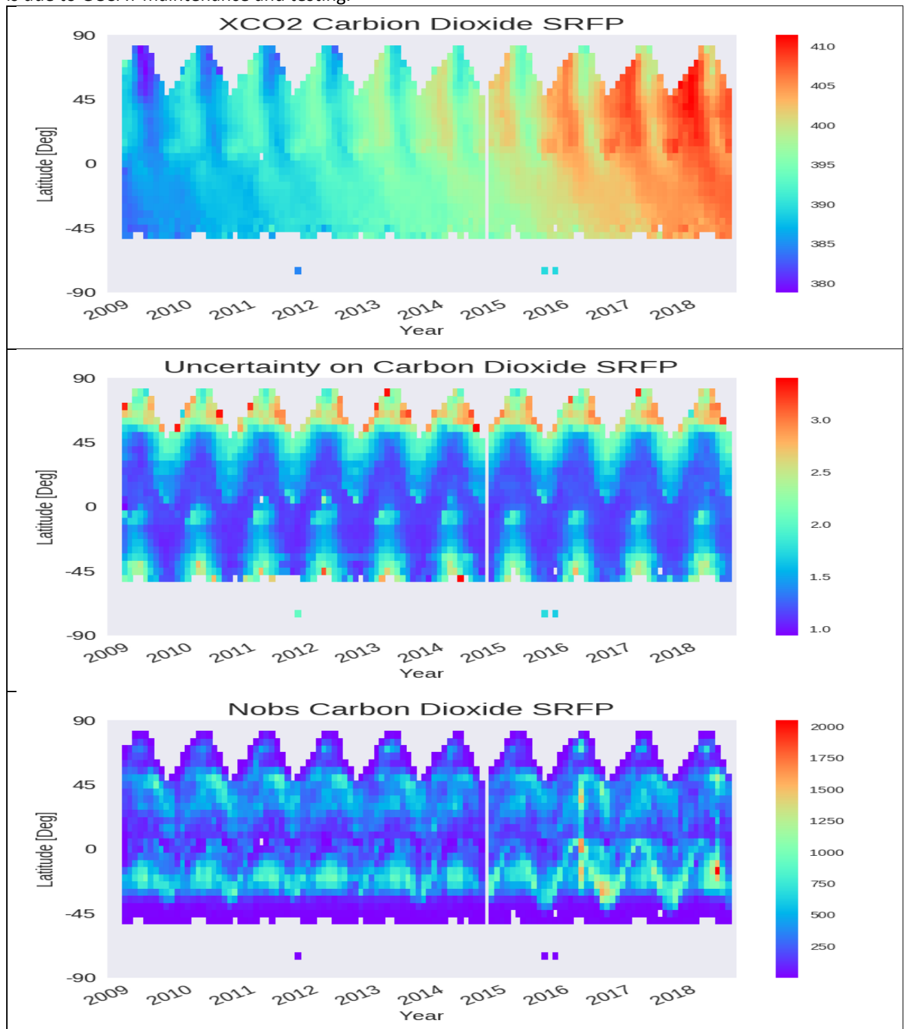
Figure 6: The CO2_GOS_SRFP global dataset in slices of 10 degrees latitude as a function of time. The yearly increase in XCO2 concentrations can clearly be seen. The gap in data coverage during Dec 2014 and Jan 2015 is due to GOSAT maintenance and testing.
