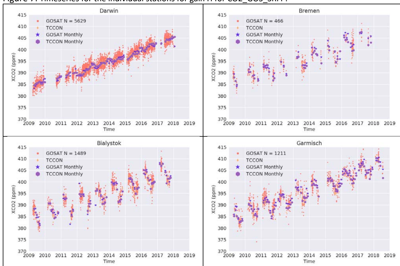
Figure 7: Timeseries for the individual stations for gain H for CO 2 _GOS_SRF.
