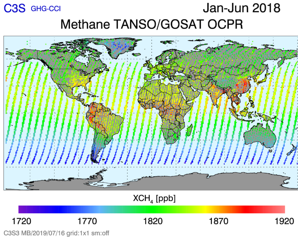
Figure 13 - XCH 4 product CH 4 _GOS_OCPR. Top: January to June 2018. Bottom: July – December 2018.
