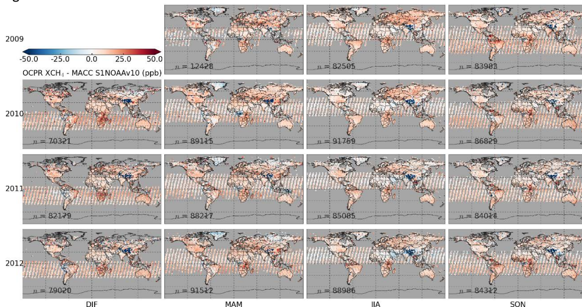
Figure 15: Seasonal means of differences between OCPv9.0 and MACC S1NOAAv10 + TOMCAT XCH 4 .
