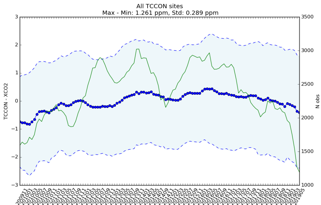
Figure 5: Year-to-year Stability of the TCCON-OCFPv7.3 XCO 2 bias calculated with \pm 6 month averaging window for each month of the GOSAT time series between April 2009 and December 2019, using the Radial co-location method. The thick blue symbols give the mean bias for a 12 month period and the shaded area indicates the standard deviation (1-sigma) of the data. The green lines give the number of data points per 12 month period.
