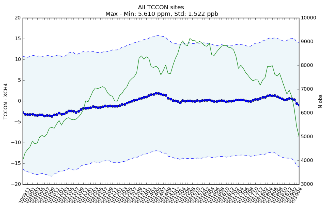
Figure 12: Year-to-year Stability of the TCCON-OCPv9.0 XCH 4 bias calculated with \pm 6 month averaging window for each month of the GOSAT time series between April 2009 and December 2018. The thick blue symbols give the mean bias for a 12 month period and the shaded area indicates the standard deviation (1-sigma) of the data. The green lines gives the number of data points per 12 month period.
