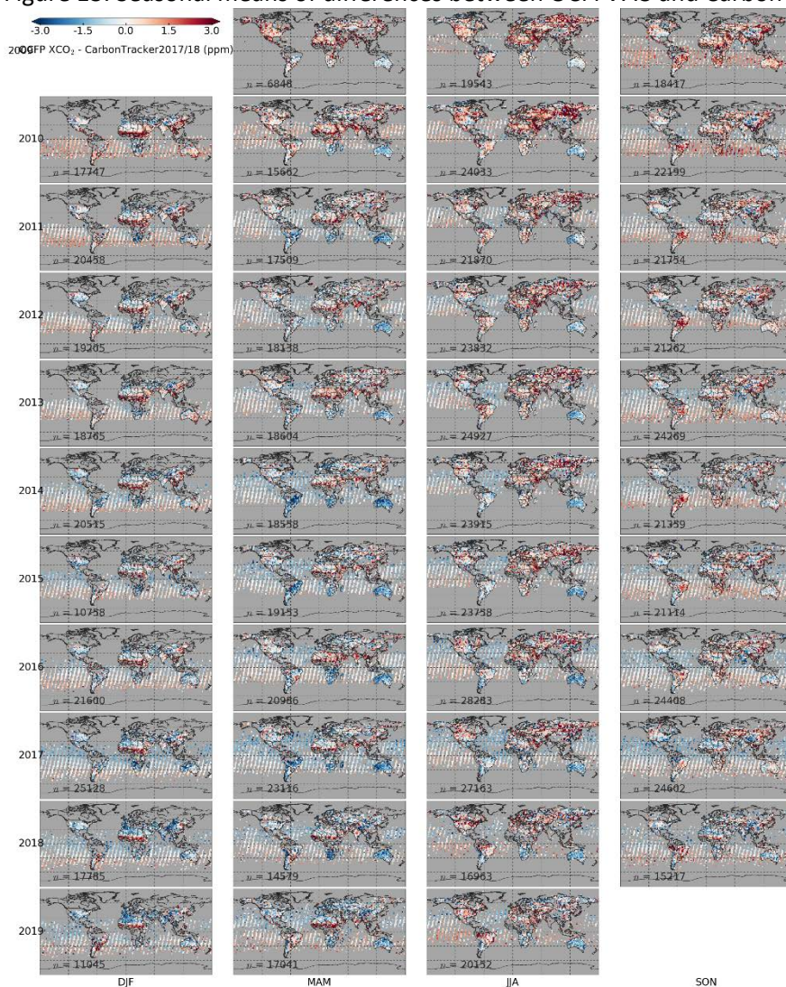
Figure 13: Seasonal means of differences between OCFPv7.3 and CarbonTracker (2017 + NRT-2018) XCO 2 .
