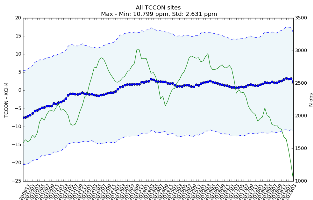
Figure 9: Year-to-year Stability of the TCCON-OCFPv7.3 XCH 4 bias calculated with for \pm 6 month averaging window for each month of the GOSAT time series between April 2009 and December 2019. The thick blue symbols give the mean bias for a 12 month period and the shaded area indicates the standard deviation (1-sigma) of the data. The green lines gives the number of data points per 12 month period.
