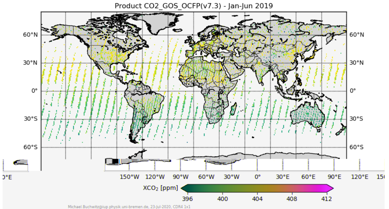
Figure 9 - XCO 2 product CO2_GOS_OCFP. Top: January to June 2019. Bottom: July – December 2019.
