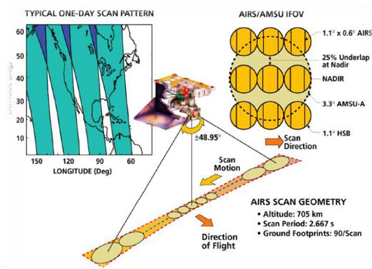
Figure 2: AIRS and AMSU scan geometrics (Jason, 2008).
