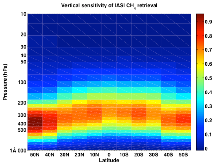
Figure 4: Vertical sensitivity of IASI CH 4 retrievals (until V8.4) as a function of latitude.
