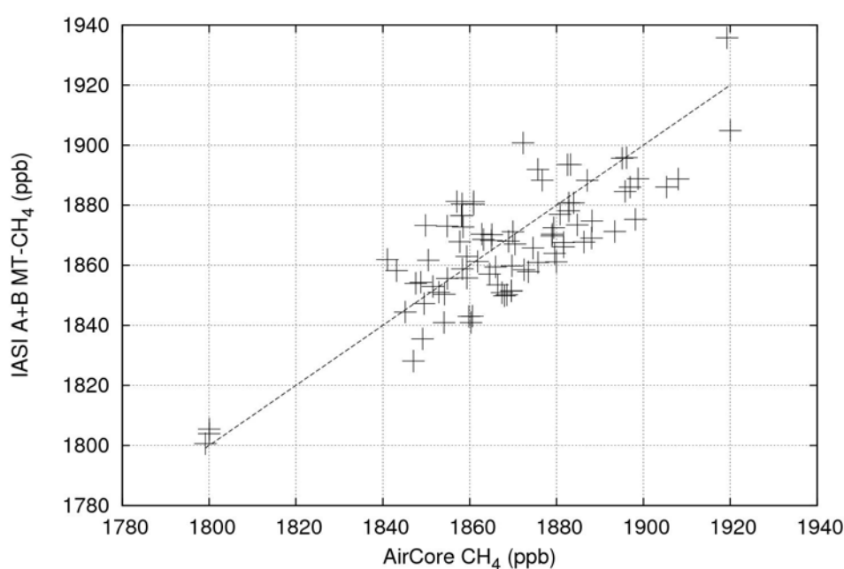
Figure 8: Comparison between IASI CH 4 v9.1 and AirCore CH 4 . Correlation is 9.1.
