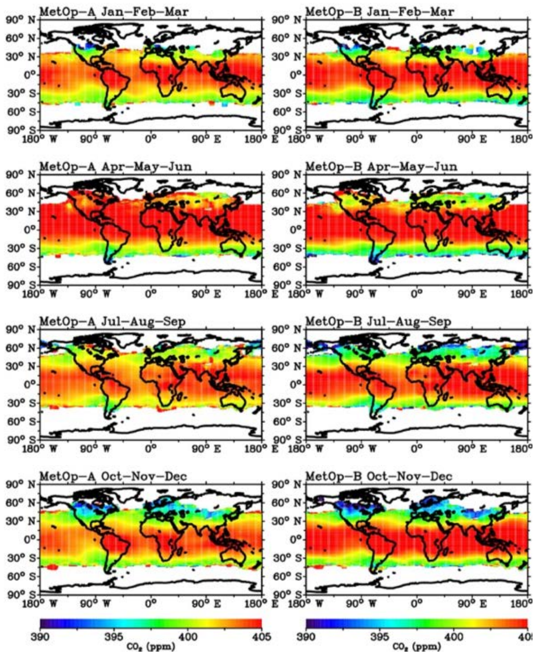
Figure 4: Seasonal maps (3 month average) of mid-tropospheric CO 2 as retrieved from Metop-A (left) and Metop-B (right), average over 2014-2021.
