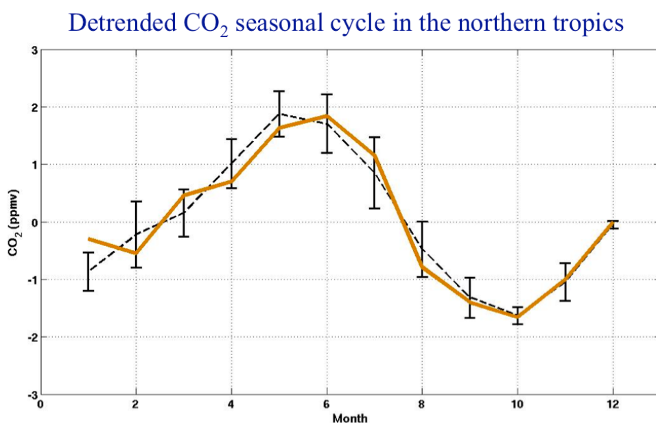
Figure 11: Detrended CO 2 seasonal cycle in the northern tropics as measured by JAL/CONTRAIL aircraft (black) and as retrieved from AIRS (brown).
