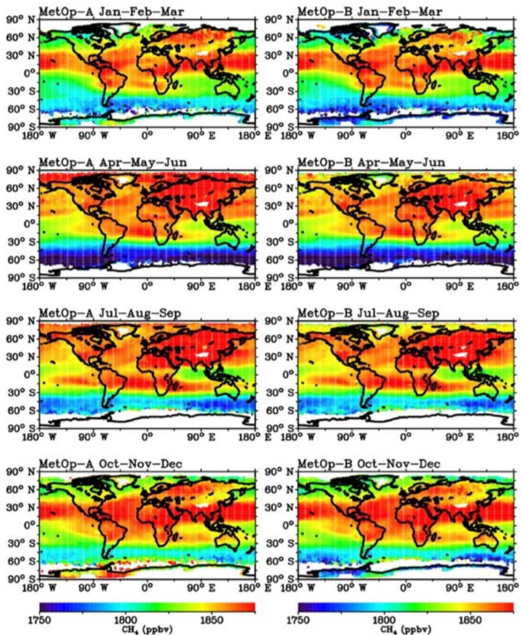
Figure 9: Seasonal maps (3 month average) of mid-tropospheric CH 4 as retrieved from Metop-A (left) and Metop-B (right), averaged over 2014-2021.
