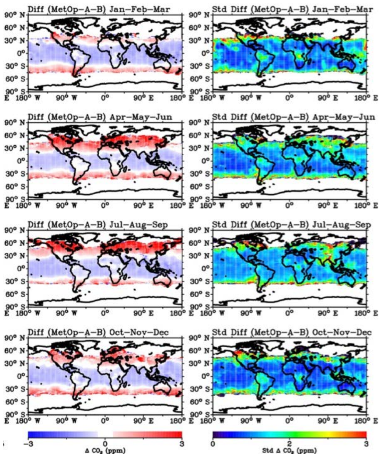
Figure 5: Seasonal maps (3 month average) of mid-tropospheric CO 2 : Mean (left) and standard deviation (right) of the difference between Metop-A and Metop-B, average over 2014-2021.
