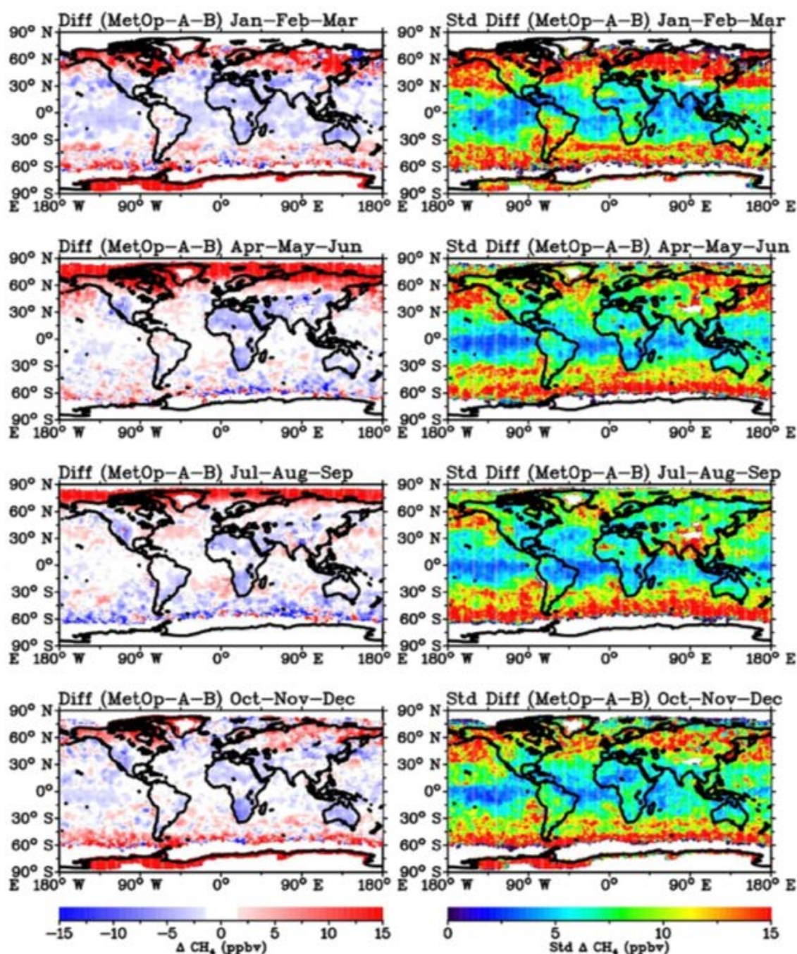
Figure 10: Seasonal maps (3 month average) of mid-tropospheric CH 4 : Mean (left) and standard deviation (right) of the difference between Metop-A and Metop-B, averaged over 2014-2021.
