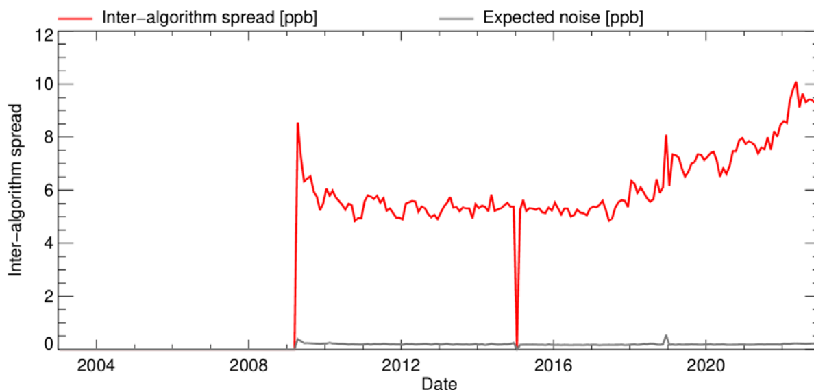
Figure 19: Monthly average of the inter-algorithm scatter and expected contribution of measurement noise.
