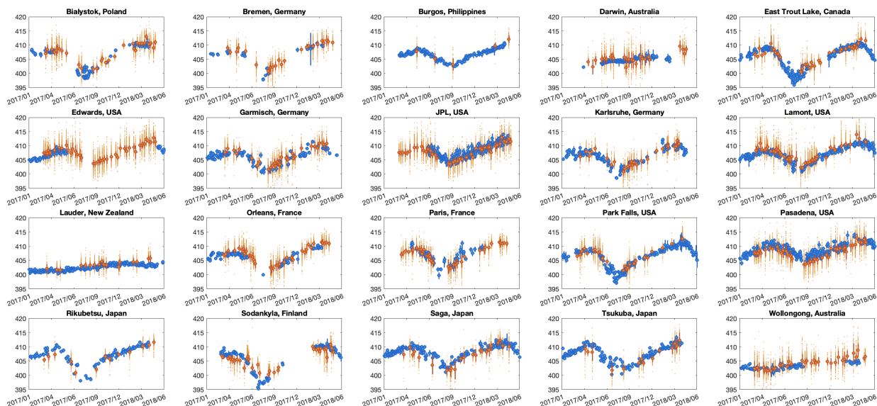
Figure 2-1. Comparison of the CO2_TAN_OCFP v1 (orange) with the TCCON XCO 2 (blue, overpass mean) between March 2017 and May 2018. The overpass-mean from TanSat is indicated with large orange solid circles with error bars indicating the standard deviation, and small orange points show individual soundings. We plot all measurements that satisfy the co-location criteria of an overpass.
