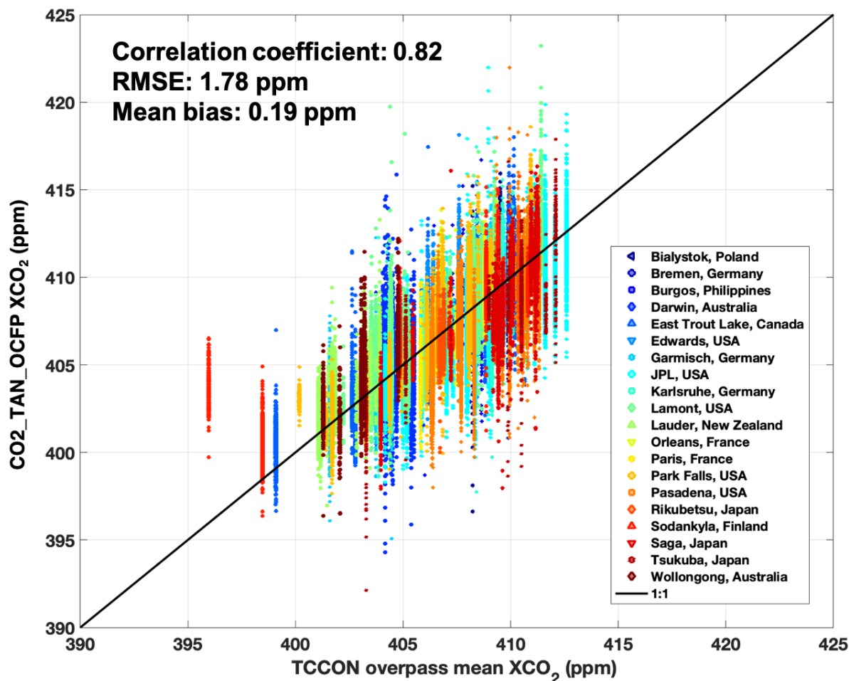
Figure 2-2. Comparison of individual retrieved XCO 2 from TanSat with the overpass mean of TCCON XCO 2 for the time period of March 2017 to May 2018 across all 20 TCCON sites. Each TCCON site is given by different colour and symbol. Statistics for mean bias and RMSE (calculated by averaging the bias and RMSE of each site) are given along with the correlation coefficient.
