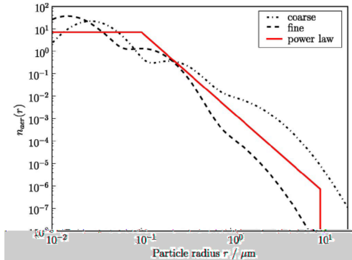
Figure 4: Aerosol size distribution n_{\text{aer}}(r) as a function of particle radius r . The retrieval method relies on a power law (red solid) size distribution. Also shown are more realistic Multi-modal lognormal size distributions for a fine mode (black dashed) and a coarse mode (black dotted) dominated aerosol type.
