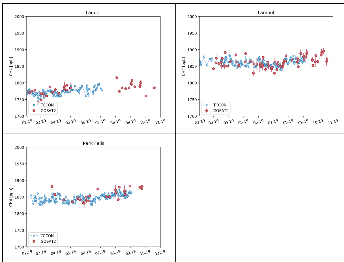
Figure 4.3 Comparison of non-glint single soundings of FP-CH 4 (red) with co-located TCCON (blue) measurements at all TCCON sites for the period Feb-Oct 2019.
