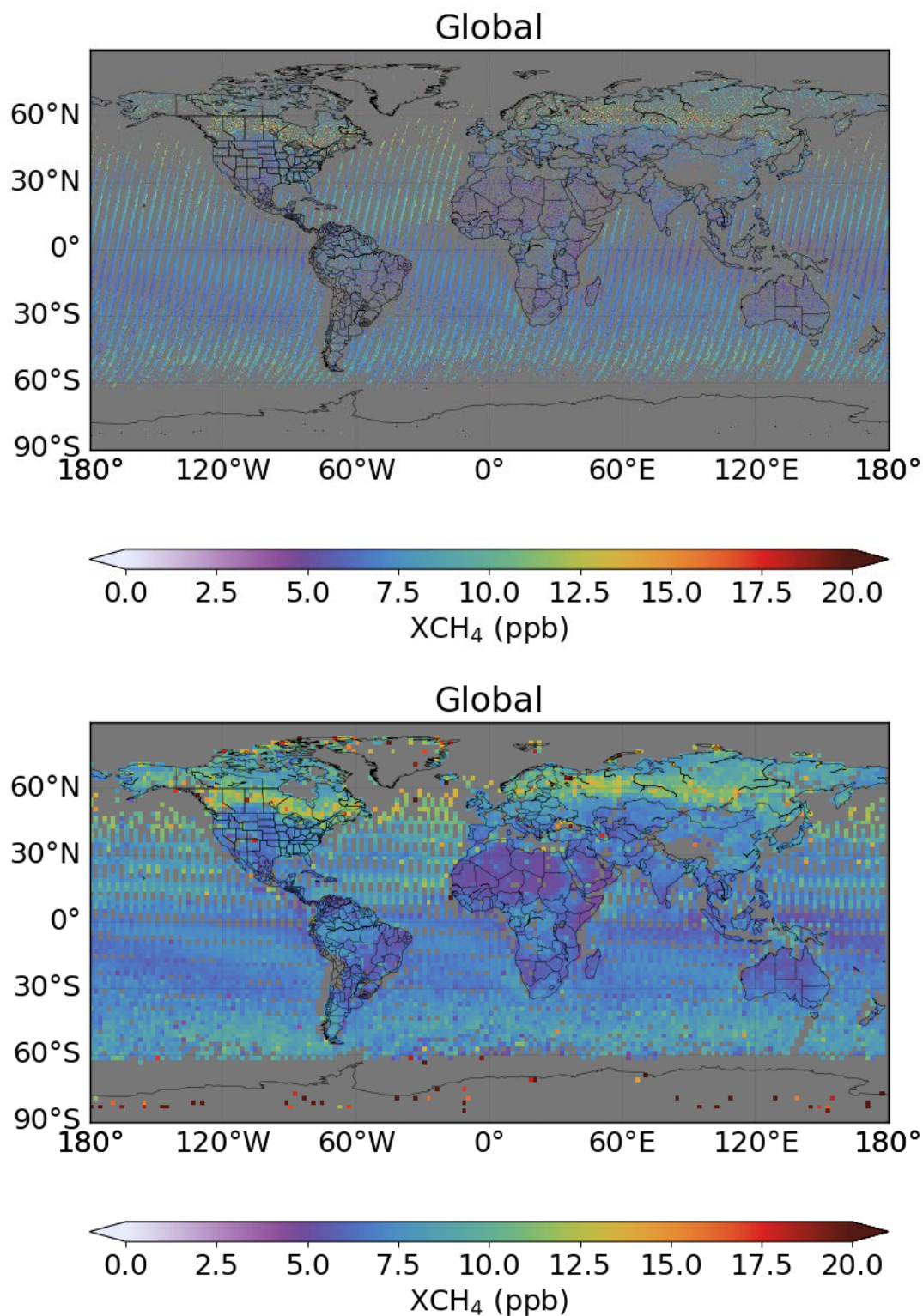
Figure 2: Same as Figure 1 but for the corresponding error.
