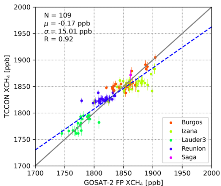
Figure 4: Validation of ocean soundings of XCH 4 with colocated TCCON measurements at all TCCON sites for the period Feb. 2019 - Dec 2021. Numbers in the figures: \mu = bias, i.e., average of the difference; \sigma = single measurement precision, i.e., standard deviation of the difference; N = number of co-locations; R = Pearson correlation coefficient.
